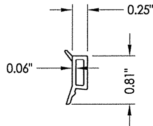
8 GLAZING BEAD Keeper Rail
