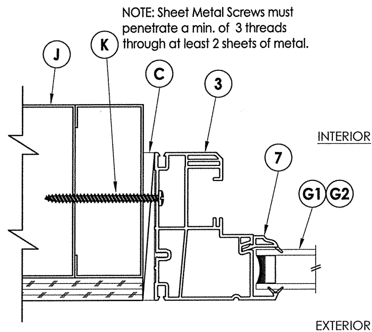
3 HORIZONTAL CROSS SECTION 2 Metal Stud Construction
