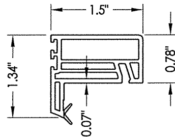
6 LOCK RAIL
