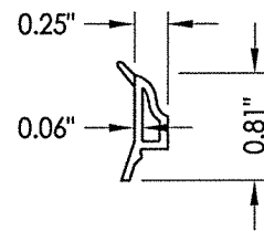
7 GLAZING BEAD Stile/ Rail
