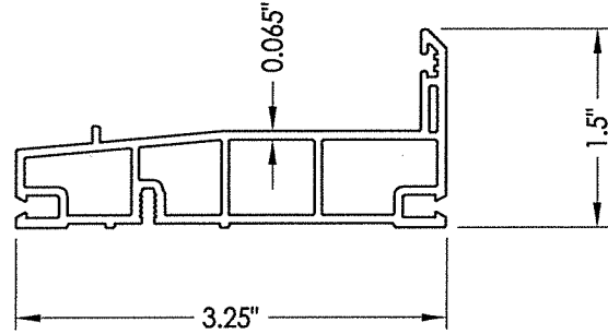
2 SILL
