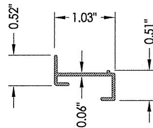
10 REINFORCEMENT
