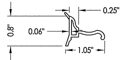
9 GLAZING BEAD Lift rail
